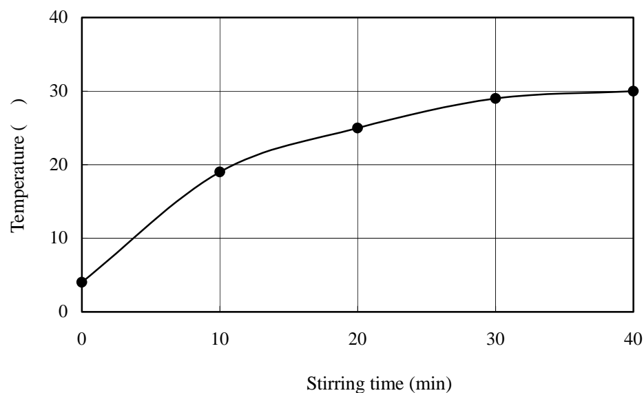
Fig.1 Stirring time and temperature rise of solder paste when using automatic stirring apparatus
